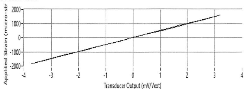
Calibration Curve
