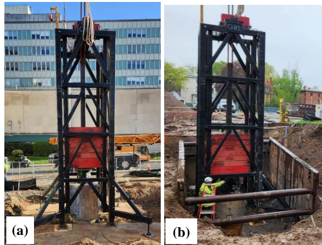
Fig. 3. Imagery of HSDLT on 3-foot-diameter caissons: (a) TS3-D1.0. (b) TS12-A3.2.
