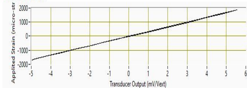
Calibration Curve
