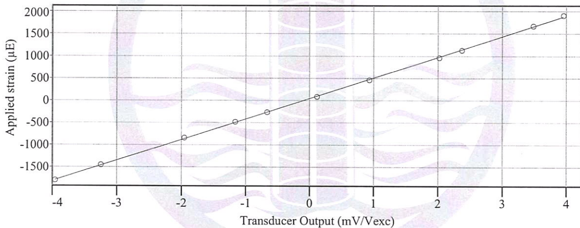
Calibration Curve
