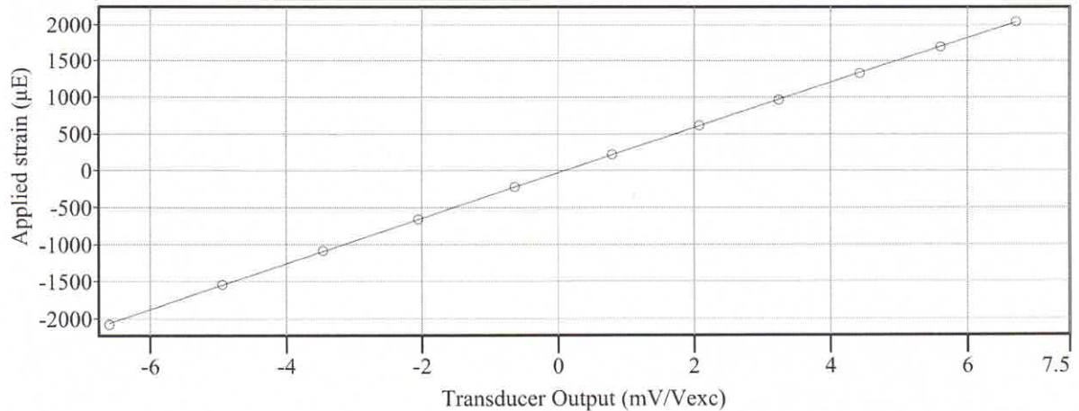
Calibration Curve
