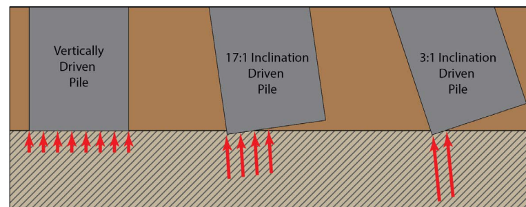
Figure 1. As the angle at which the pile encounters bedrock becomes more severe, the localized stresses become greater over a smaller area of the pile's cross-section increasing the likelihood of pile damage.
