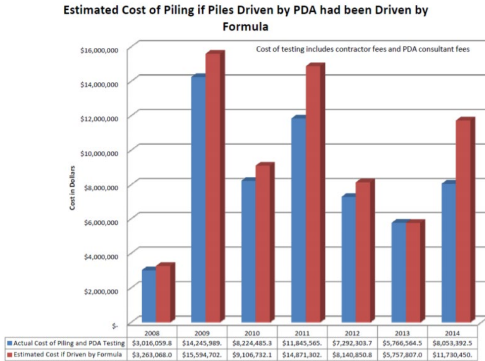
Figure 1. Summary of Pile Installation Costs, Indiana 2008 - 2014
