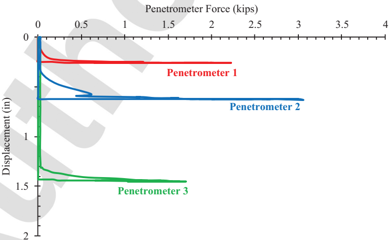
FIG. 4 Force-displacement plot from SQUID testing.
