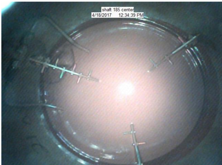
FIG. 2 Mini-SID at the bottom of a drilled shaft.
