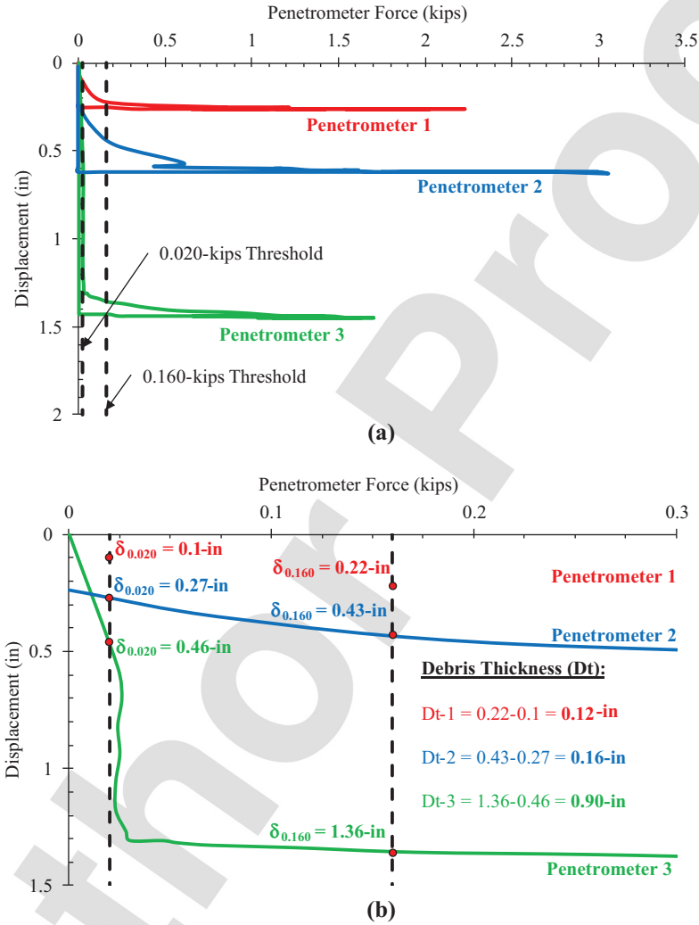
FIG. 5 Debris thickness from SQUID testing: (a) overall thresholds and (b) debris thickness calculation.
