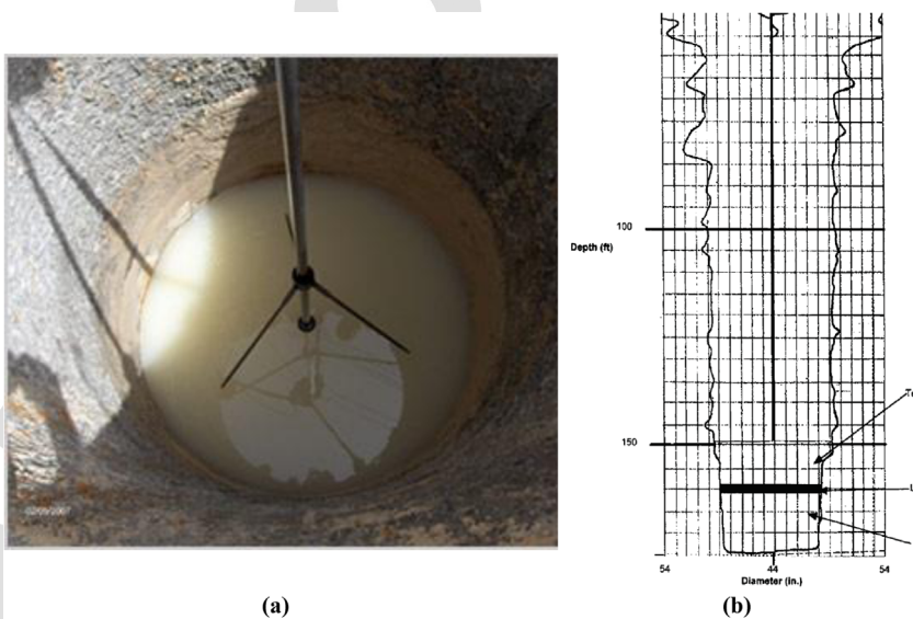
FIG. 10 Mechanical caliper (a) during testing and (b) testing results.
