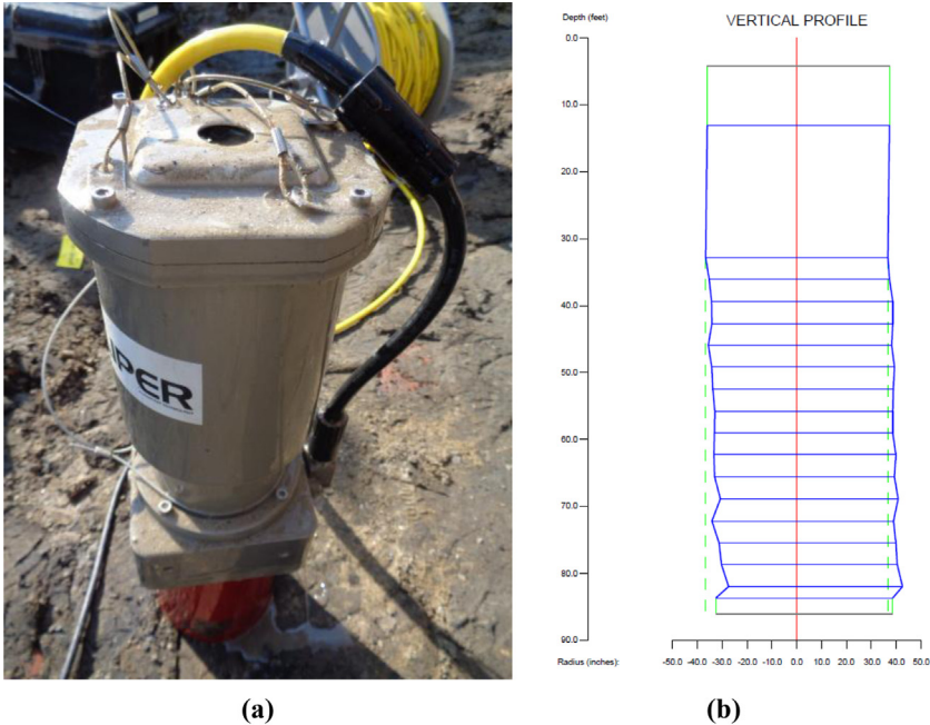
FIG. 11 Sonar caliper (a) before testing and (b) testing results.
