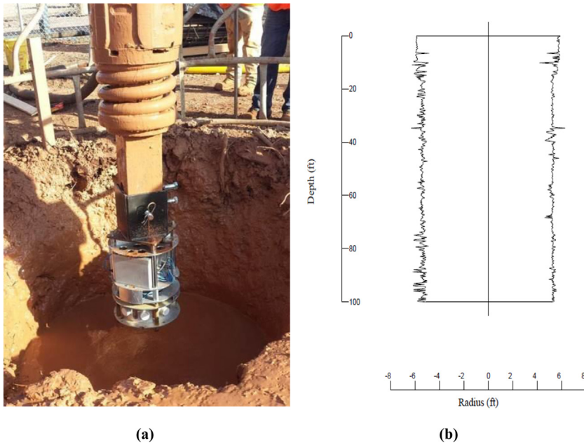
FIG. 12 SHAPE (a) before testing and (b) testing results.
