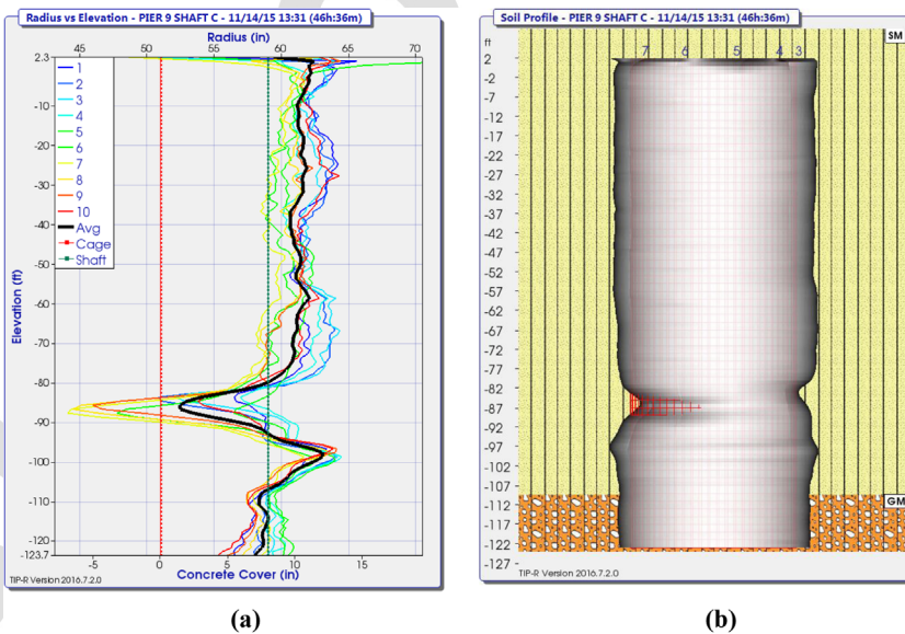
FIG. 7 Thermal integrity profiling wire results for a defective drilled shaft: (a) effective radius versus elevation and (b) three-dimensional model overlaying the soil profile.
