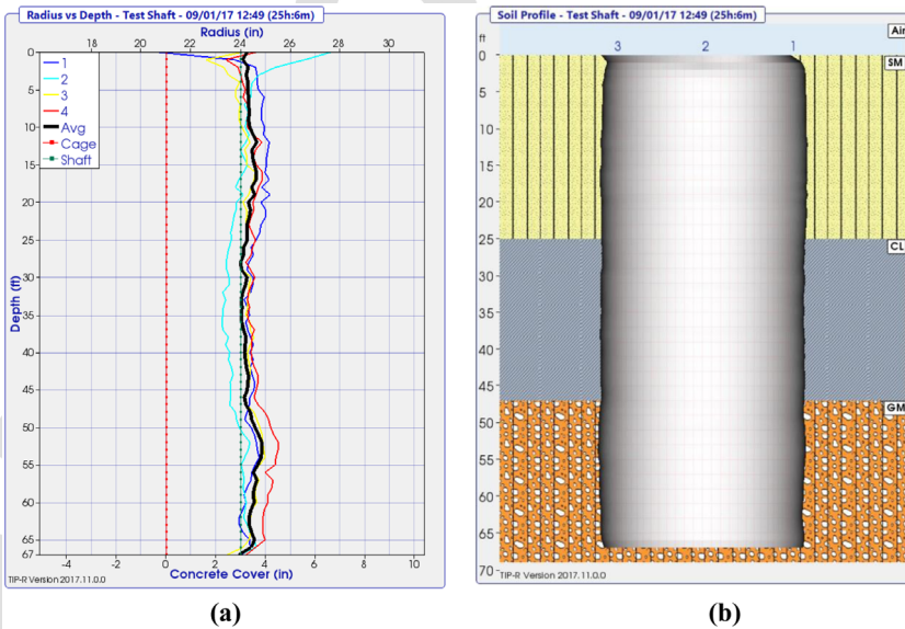
FIG. 6 Thermal integrity profiling results for a satisfactory drilled shaft: (a) effective radius versus depth and (b) three-dimensional model overlaying the soil profile.
