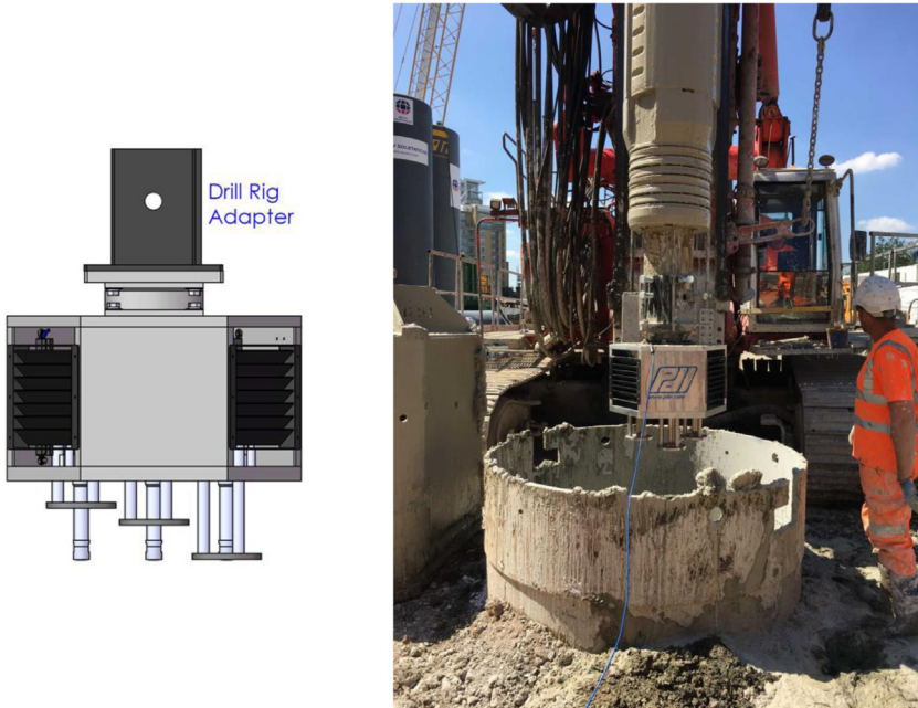
FIG. 3 SQUID sr : Shaft Quantitative Inspection Device (SQUID)
