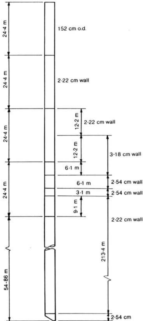
Fig. 7. Jacket pile details
