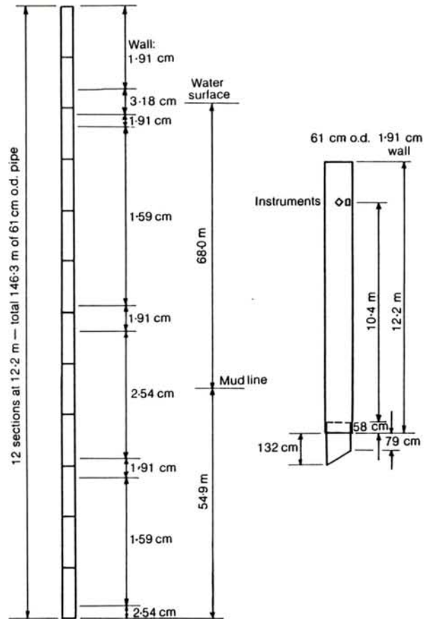
Fig. 4. Conductor pipe details
