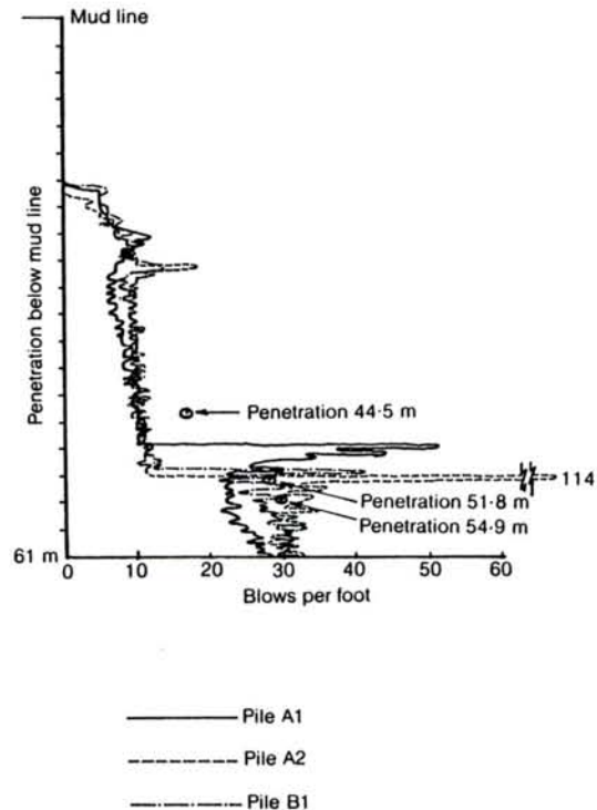
Fig. 8. Driving records for jacket piles
