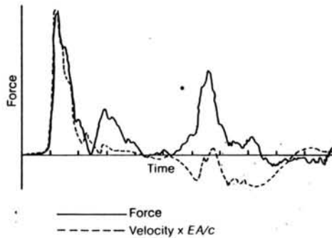
Fig. 2. Example of force and velocity record
