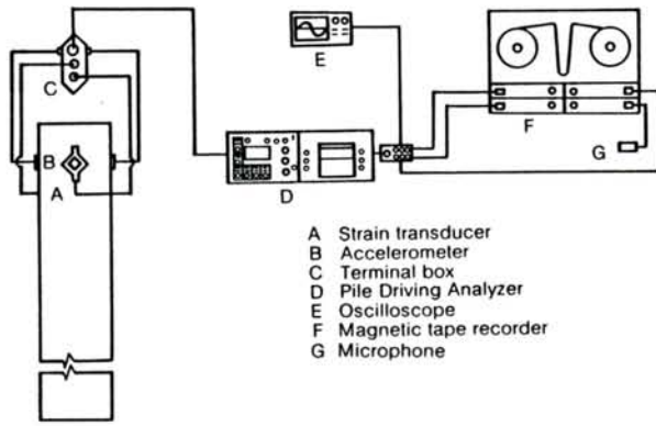
Fig. 1. Pile driving data acquisition system
